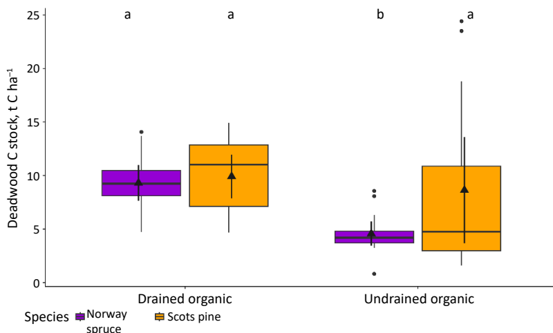
Figure 3.1 Mean deadwood carbon stock by soil type in spruce and pine stands
