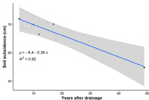
Figure 3. Differences in soil subsidence at various times after forest drainage at Myrtilloso turf. mel. (Mmel) sites.
